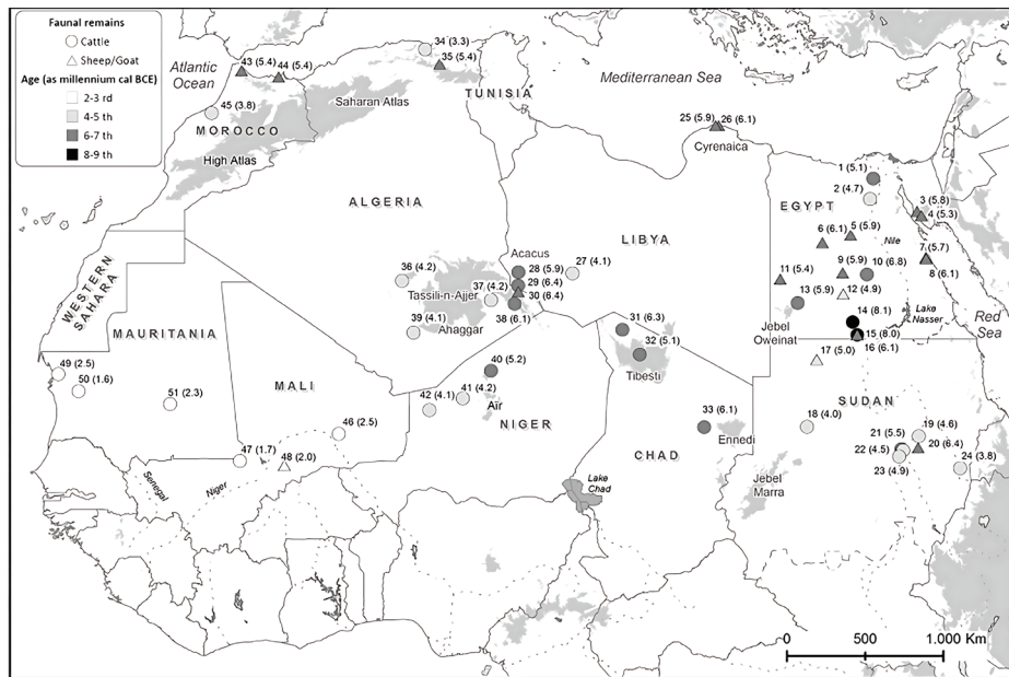
FIGURE 1. Map of principal North African sites with earliest presence of cattle (dot) and sheep/goat (triangle). Radiocarbon dates have been calibrated (OxCal 4.2) and the average age of each site is reported in brackets (e.g., 7.3 = 7300 calBCE). Sites are numbered according to country and by latitude:
